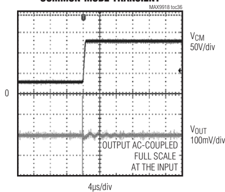
OUTPUT RESPONSE TO COMMON-MODE TRANSIENT
