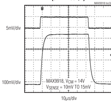
SMALL-SIGNAL TRANSIENT (GAIN = 90V/V)
